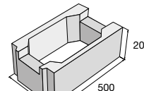
ZB 20-40
