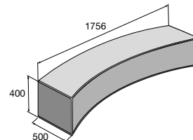
LEDGE 9
