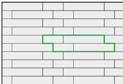
FERRA 1 - 3,33 ks/m 2 , 66,67% dl. plochy FERRA 2 - 3,33 ks/m 2 , 33,33% dl. plochy
