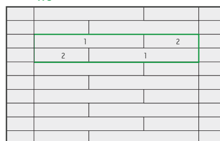
WOODY 1 - 2,08 ks/m 2 , 66,67% dl. plochy WOODY 2 - 2,08 ks/m 2 , 33,33% dl. plochy
