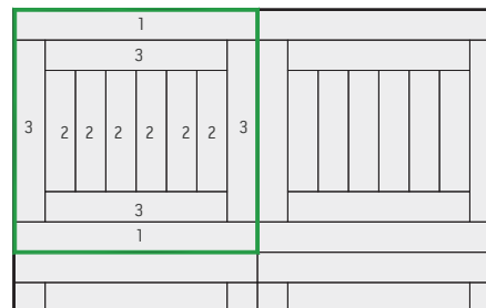
WOODY 1 - 0,78 ks/m 2 , 25% dl. plochy WOODY 2 - 2,34 ks/m 2 , 37,5% dl. plochy WOODY 3 - 1,56 ks/m 2 , 37,5% dl. plochy
