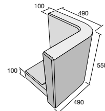
STANDARD S 55 VR 90 O
