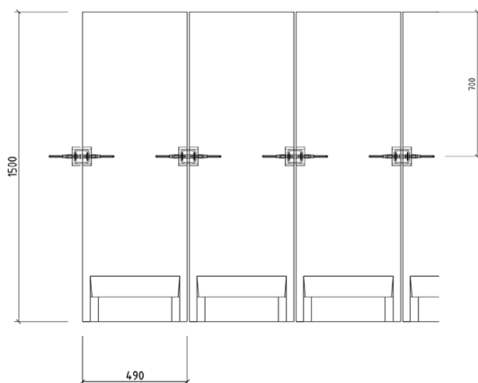
STANDARD S150 Pohled
