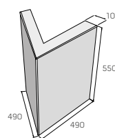
STANDARD VR 60°
