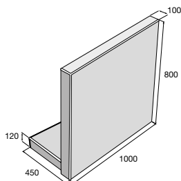
STANDARD S 55/R, relief – prkno
