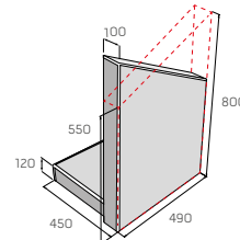
STANDARD S 120
