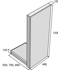
STANDARD S 120
