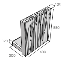
STANDARD S 55/R, relief – prkno
